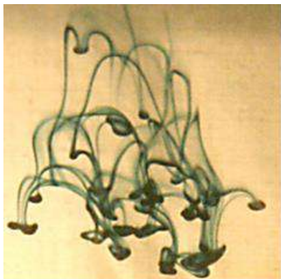
Multi-tiered vortex cascade of a falling drop
